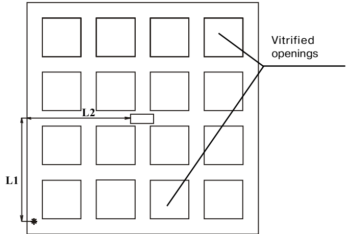
Fig.6 Monitoring a window frame
