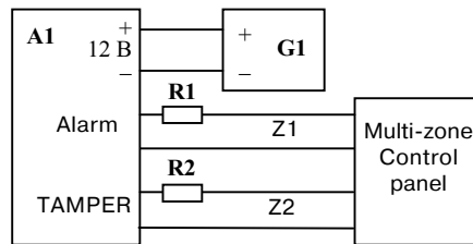
Fig. 2. Wiring diagram of the sensor with separated "Alarm" and "Tamper" signals.
