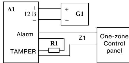
Fig. 1. Wiring diagram of the sensor with combined "Alarm" and "Tamper" signals.
